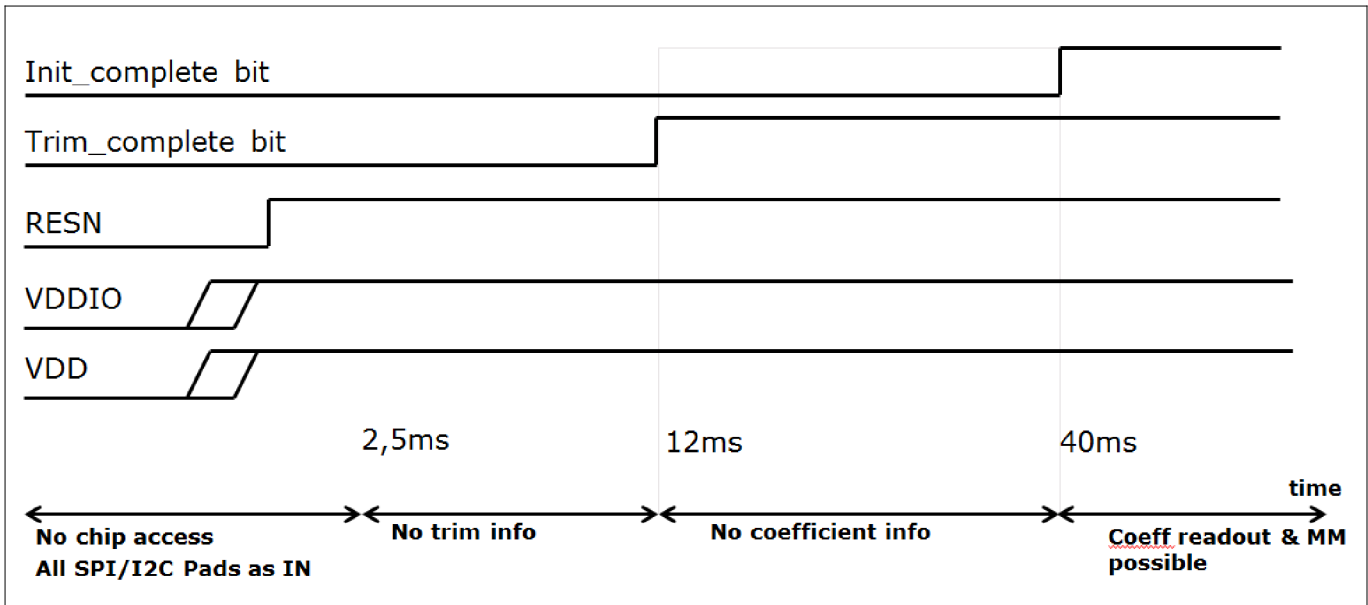
Figure 4 Start-up sequence
